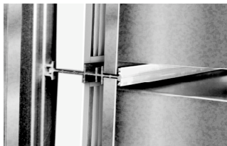
Polyseal housing shown with PerfectPleat® prefilter and VariCel® final filter. The Polyseal System includes an extruded aluminum mounting track and final filter gaskets with space for static taps.
