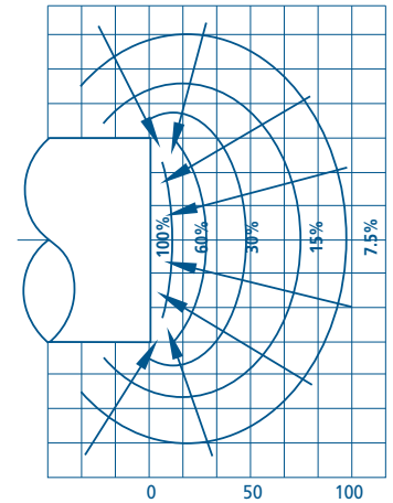
Figure 1 - % OF DIAMETER VELOCITY CONTOURS As per Industrial Ventilation Recommended Practices Standard, the larger the opening, the greater the capture area, the more efficient your particle capture.
